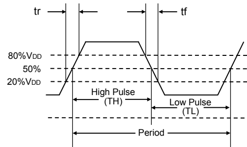
FIGURE 2. WAVEFORM
