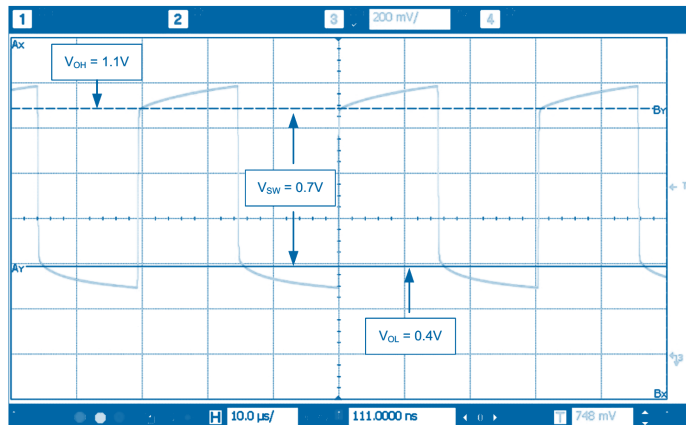
FIGURE 13. PROGRAMMABLE OUTPUT SWING WAVEFORM ( V_{OH} = 1.1V , V_{OL} = 0.4V ; ULPO-RB2)
